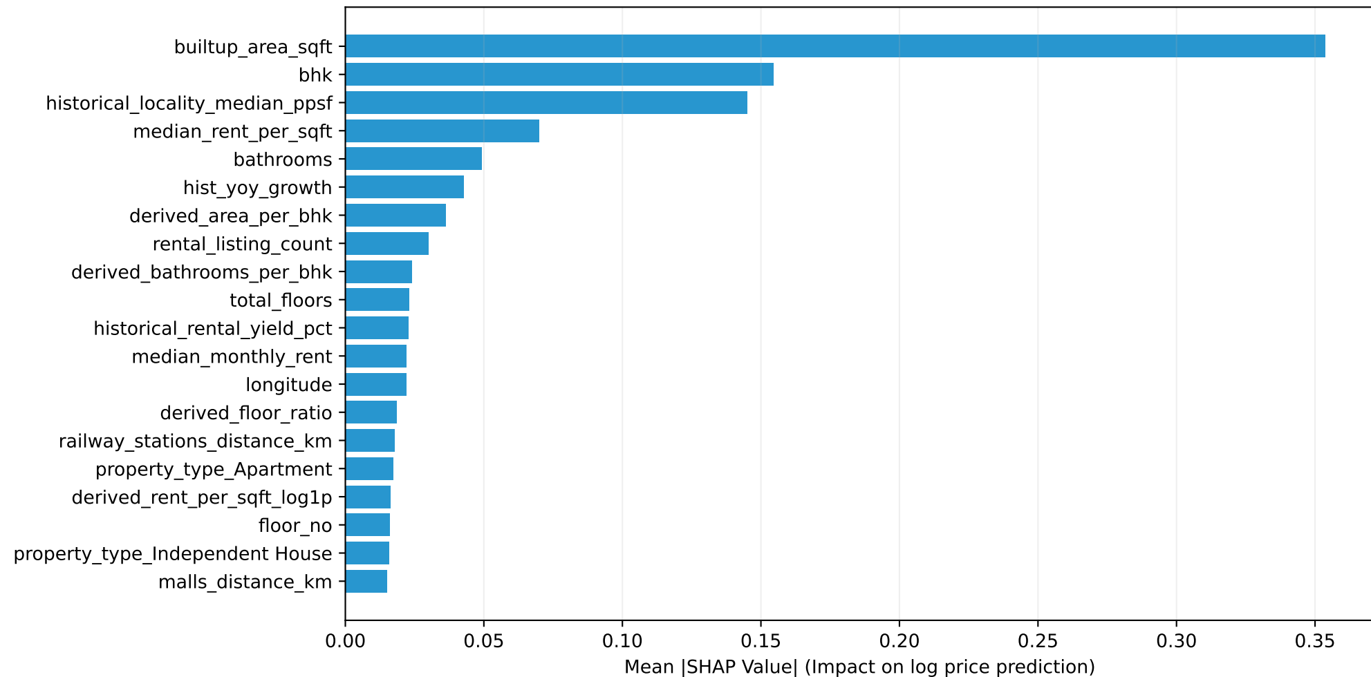
Top 20 Feature Importance by Mean |SHAP Value|
