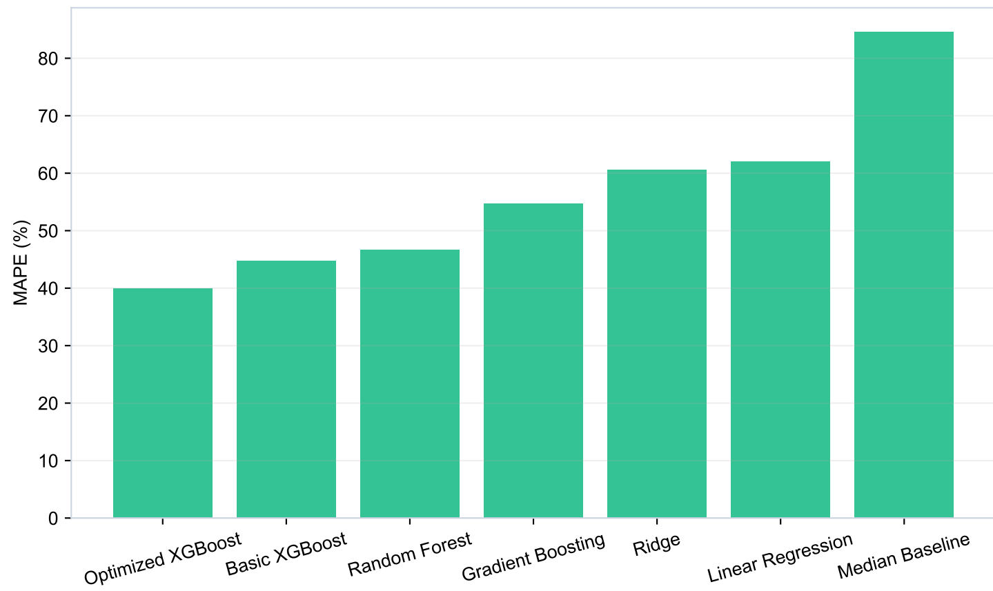
Figure 12D: Model Performance Comparison — MAPE (Temporal Test Set)
