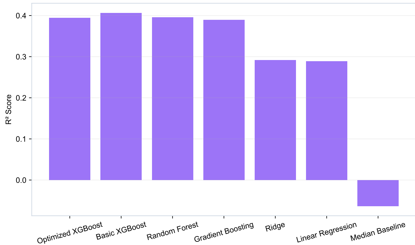
Figure 12C: Model Performance Comparison — R^2 Score (Temporal Test Set)
