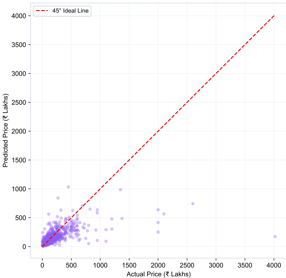
Figure 13: Actual vs Predicted Price (Optimized XGBoost v4)
