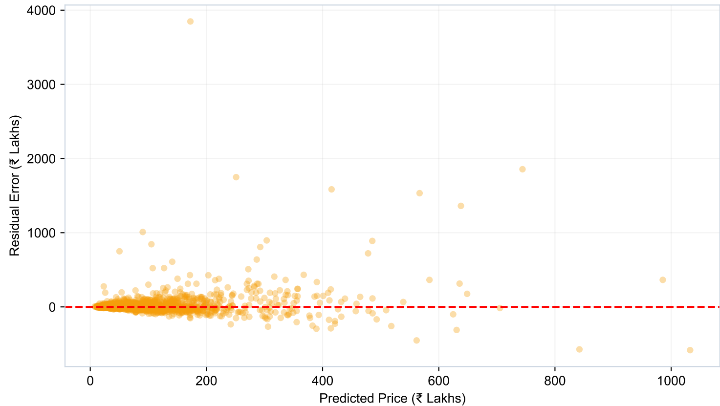
Figure 14B: Residual Error vs Predicted Price
