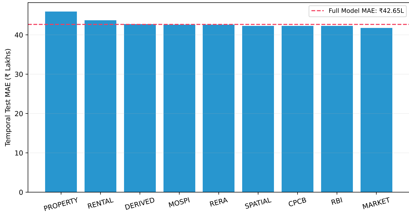
Figure 1: Leave-One-Group-Out Ablation Impact on MAE (Higher = More Important)
