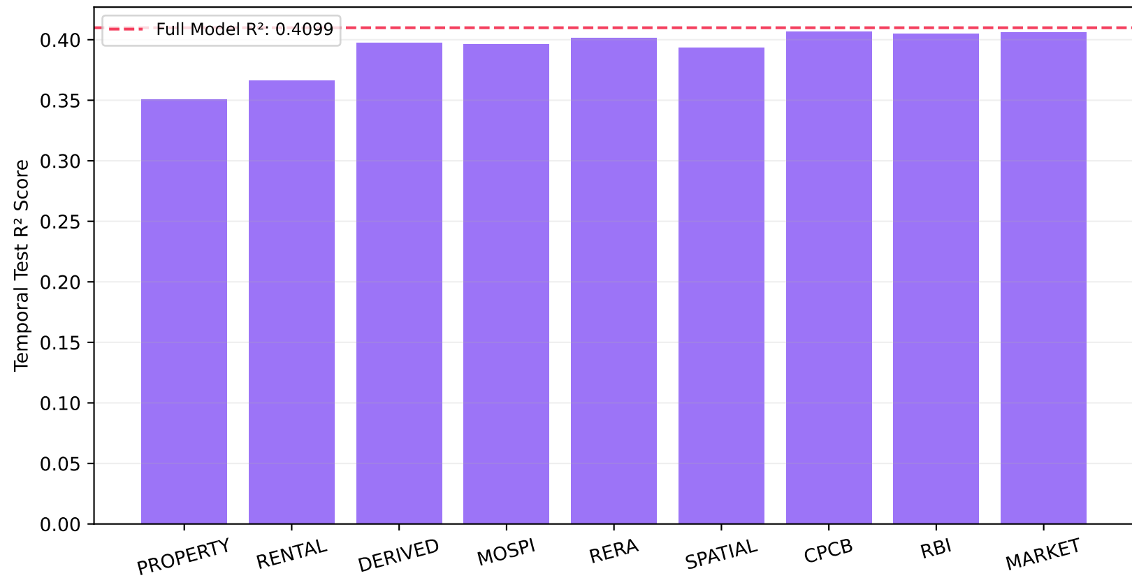
Figure 3: Leave-One-Group-Out Ablation Impact on R 2 Score (Lower = More Important)
