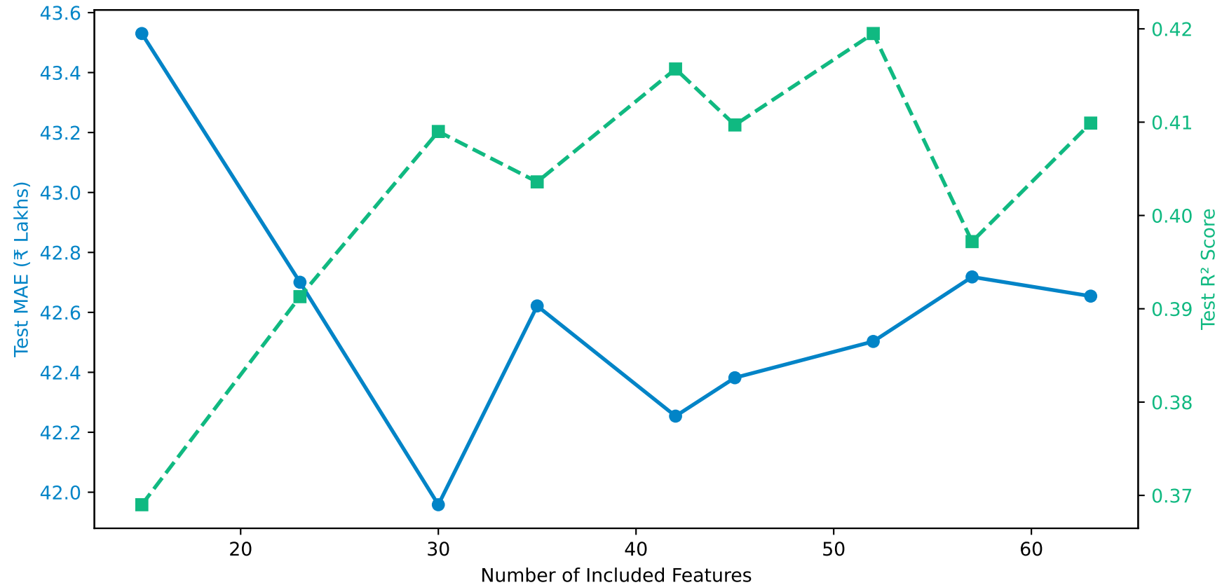
Figure 4: Cumulative Feature Addition vs Predictive Performance
