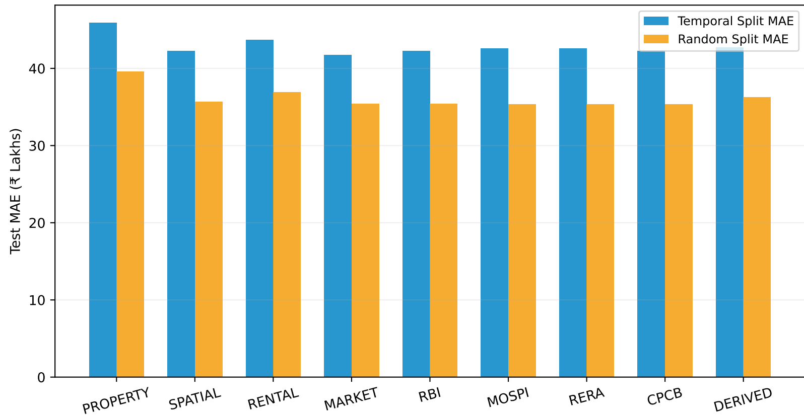
Figure 6: Temporal vs Random Split Ablation Comparison
