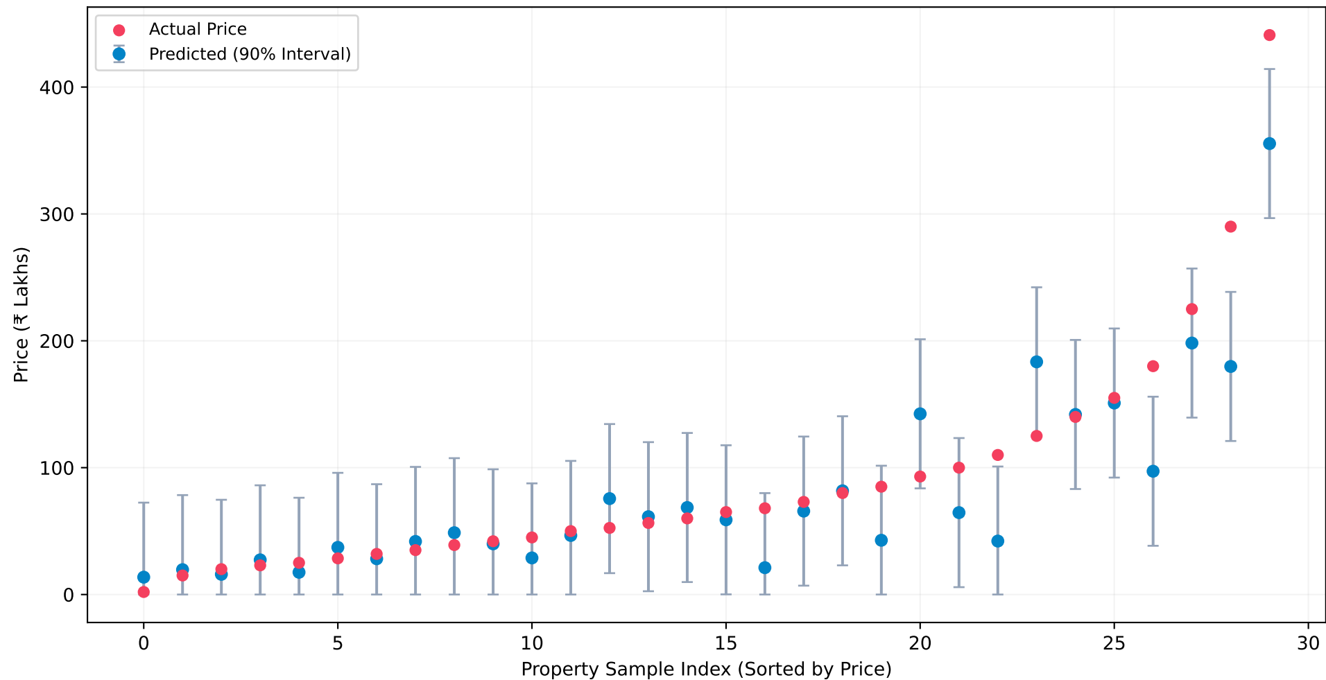
Figure 1: 90% Conformal Prediction Intervals for Representative Test Properties
