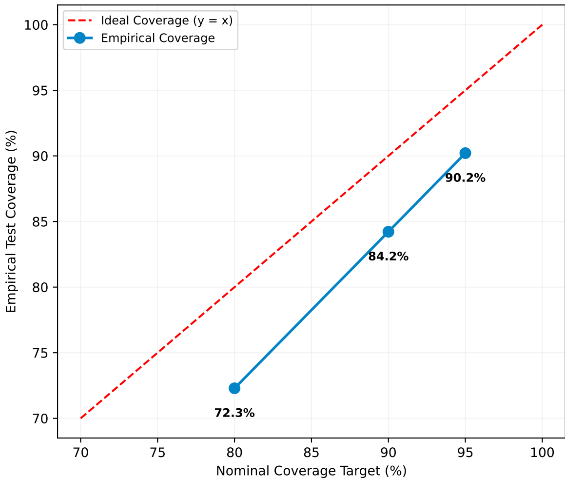
Figure 2: Conformal Calibration: Nominal vs Empirical Coverage
