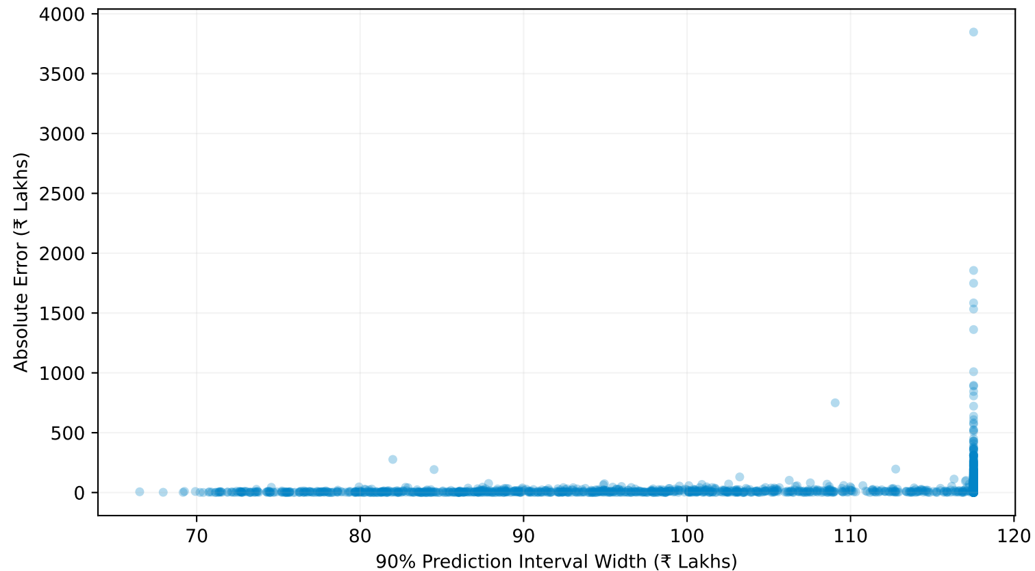
Figure 7: Absolute Prediction Error vs 90% Interval Width (Pearson r = 0.18 )
