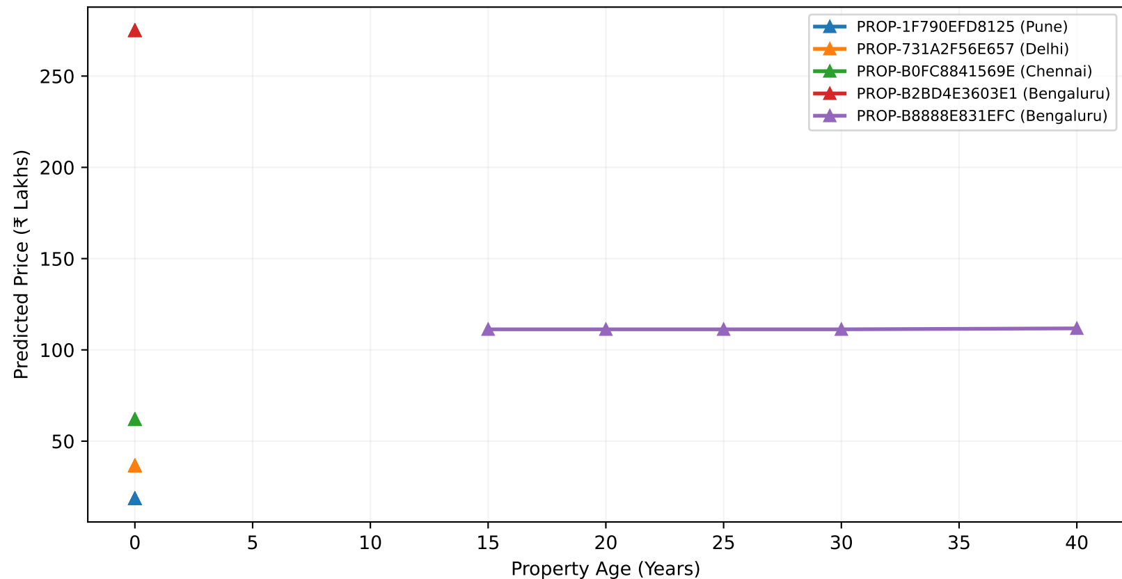
Figure 3: Model Prediction Sensitivity to Property Age
