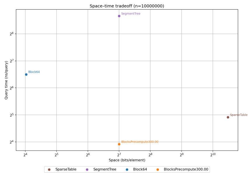
Figure 3 space-time trade-off
