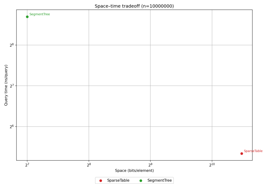
Figure 3 space-time trade-off
