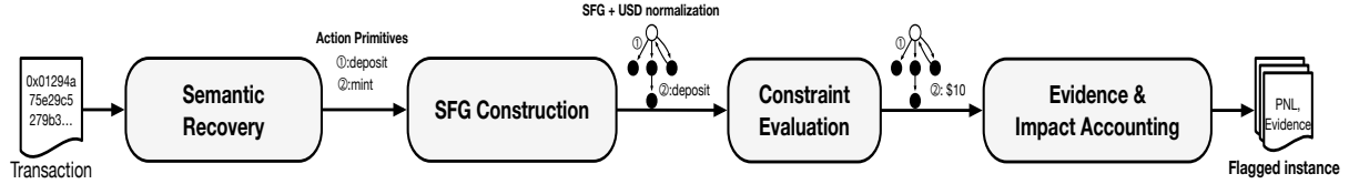
Fig. 1. Measurement pipeline. Evanescence performs semantic recovery, constructs USD-normalized SFGs, evaluates DSL constraints, and outputs replayable evidence traces.
