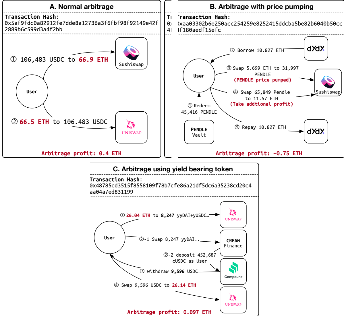
Fig. 3. Arbitrage patterns at scale (RQ2), from benign baseline (Panel A) to non-baseline variants: price pumping (B) and yield-token cross-protocol paths (C).
