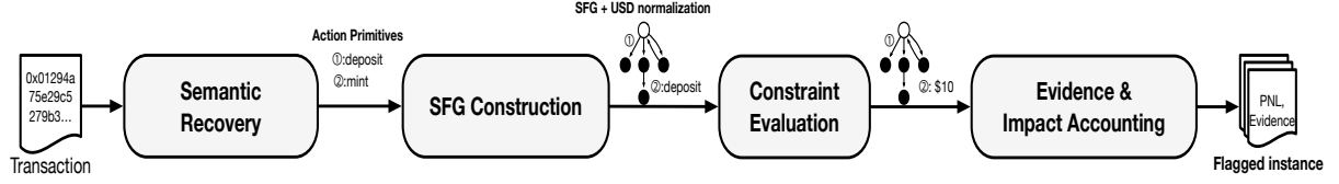
Fig. 1. Measurement pipeline. Evanesca performs semantic recovery, constructs USD-normalized SFGs, evaluates DSL constraints, and outputs replayable evidence traces.
