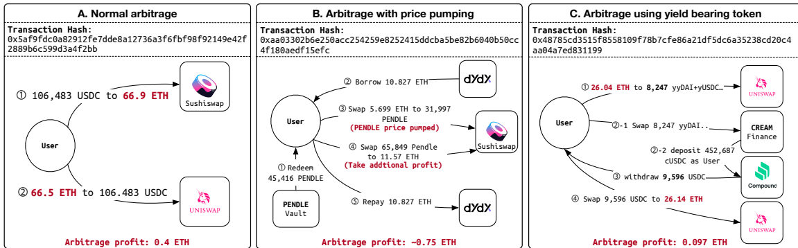
Fig. 3. Representative arbitrage patterns used for the RQ2 classification: routine arbitrage baseline (A), price pumping (B), and yield-bearing token deviation (C).
