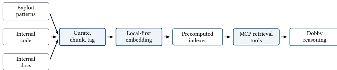
Fig. 2. Dobby’s RAG composition. Vulnerability, repository, and documentation memories are curated and embedded into bounded indexes, then exposed through MCP tools rather than pasted directly into prompts.
