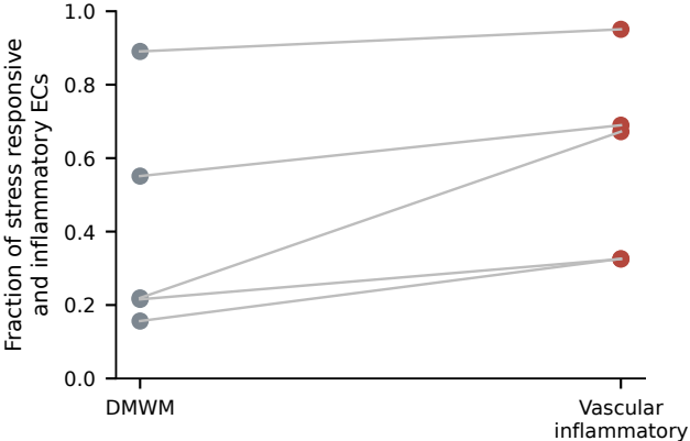
F GSE284005 endothelial composition
