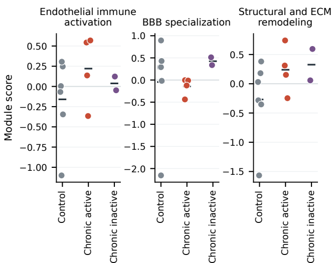
C BBB modules in MS inflammatory microenvironments
