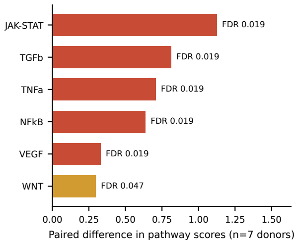
B Pathways in MS inflammatory microenvironments
