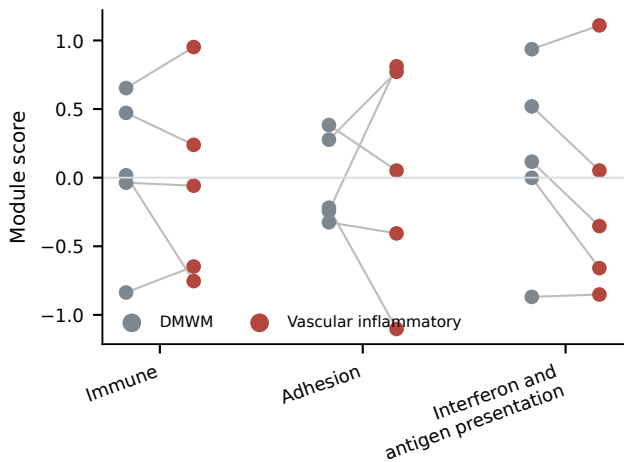
E GSE284005 paired endothelial programs
