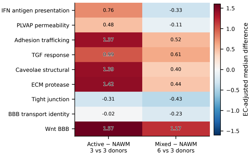
D GSE208747 lesion stage sensitivity
