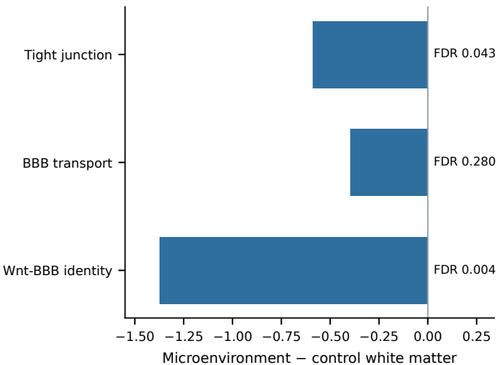
C BBB modules in MS inflammatory microenvironments
