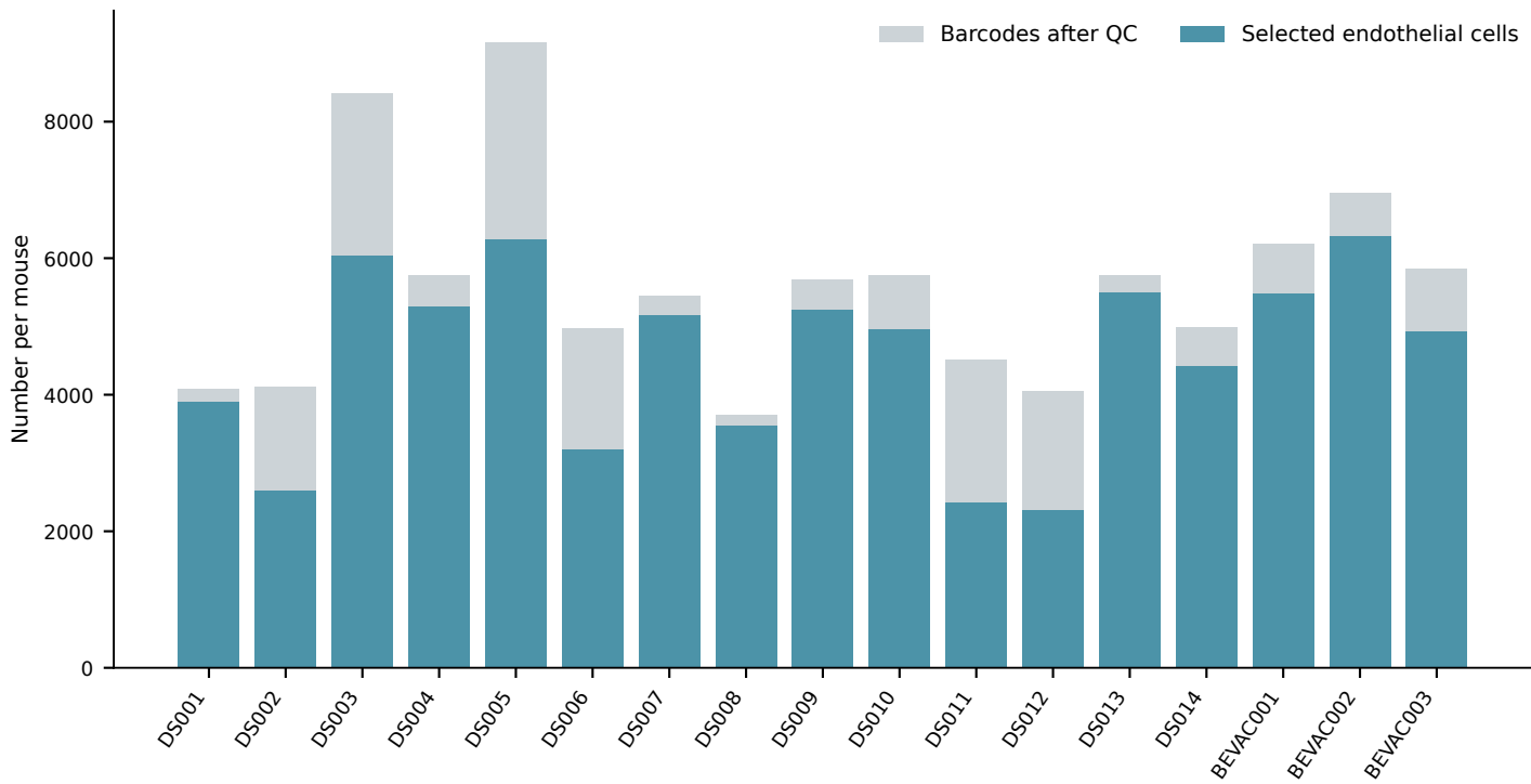
A GSE210776 raw-droplet filtering and endothelial-cell yield
