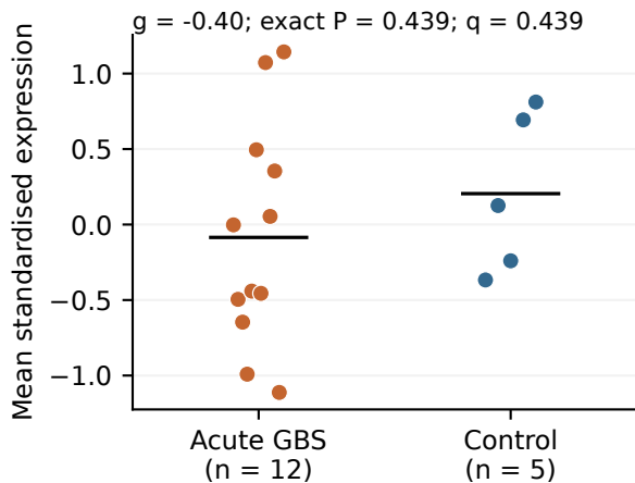
A CXCL8 recruitment · acute comparison
