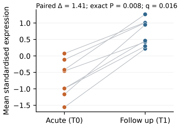
C CXCL8 recruitment · paired follow up
