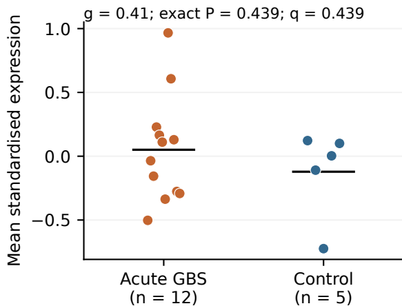
B Complement · acute comparison
