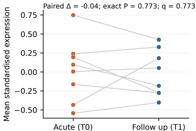
D Complement · paired follow up
