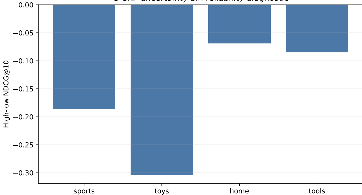
C-CRP uncertainty-bin reliability diagnostic
