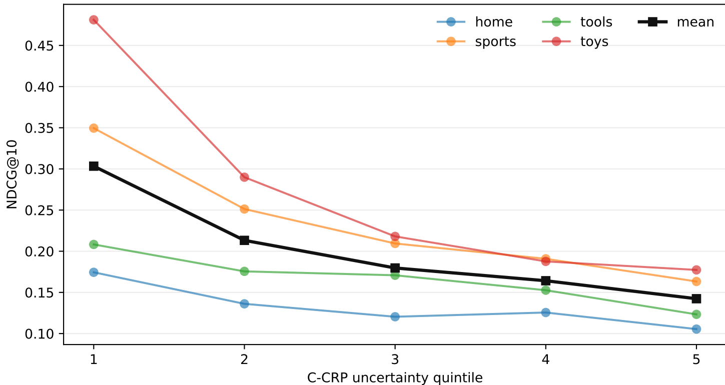
Reliability across C-CRP uncertainty bins
