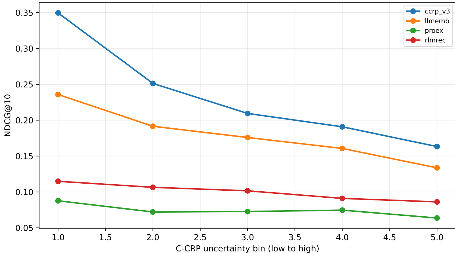
Uncertainty-motivation diagnostic
