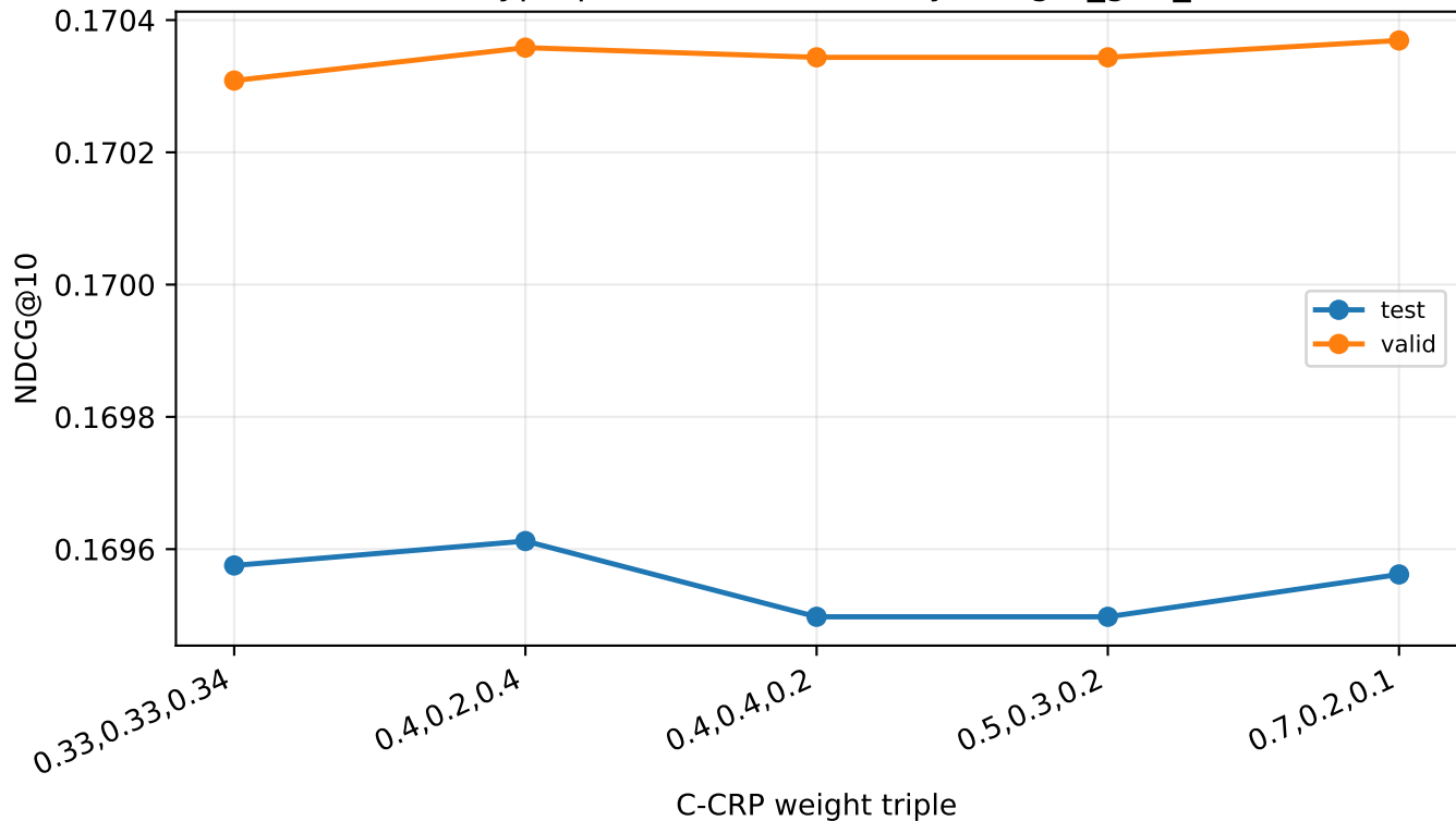
C-CRP hyperparameter sensitivity: weight_grid_label
