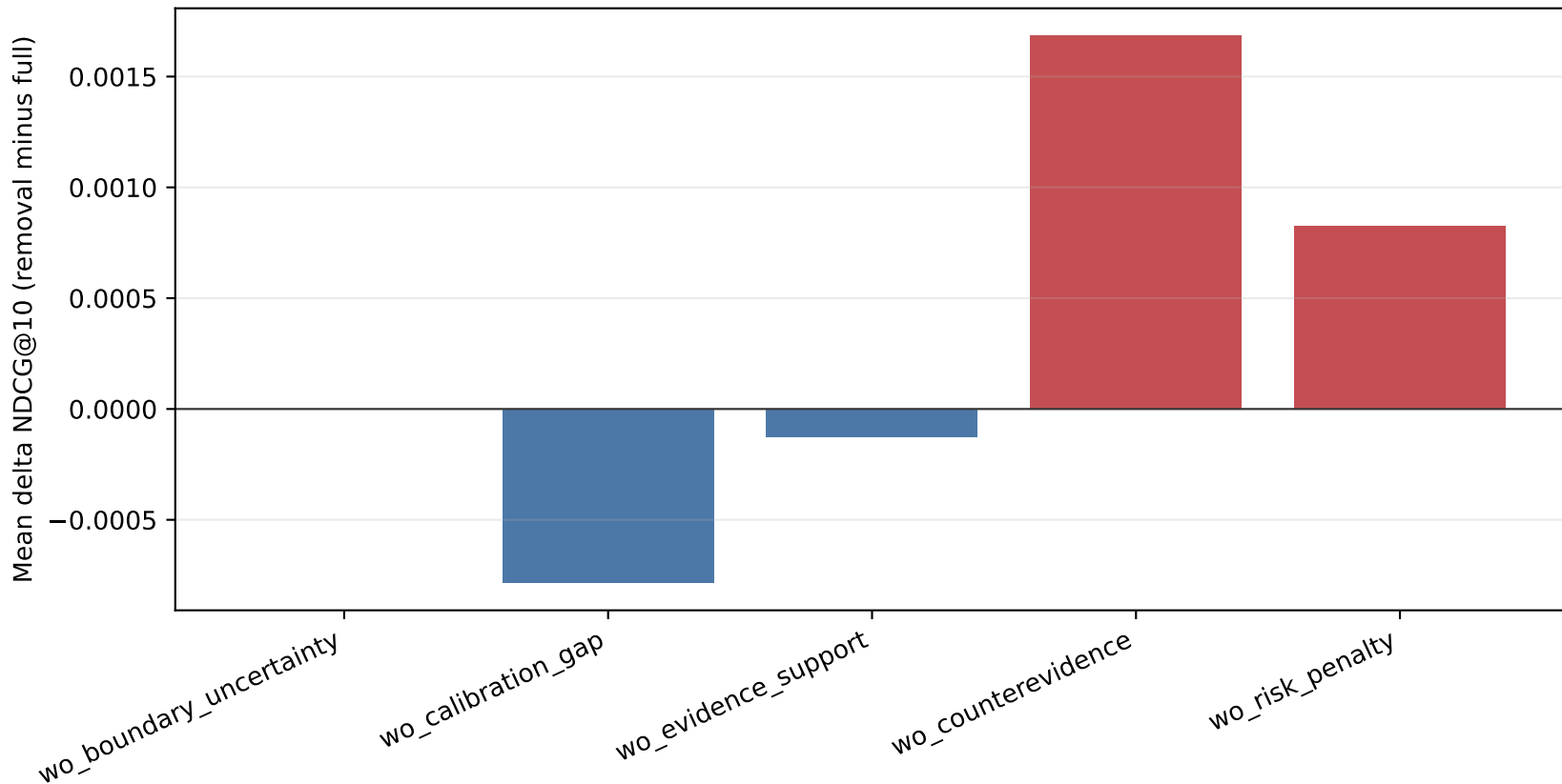
C-CRP component ablation across full-scale domains
