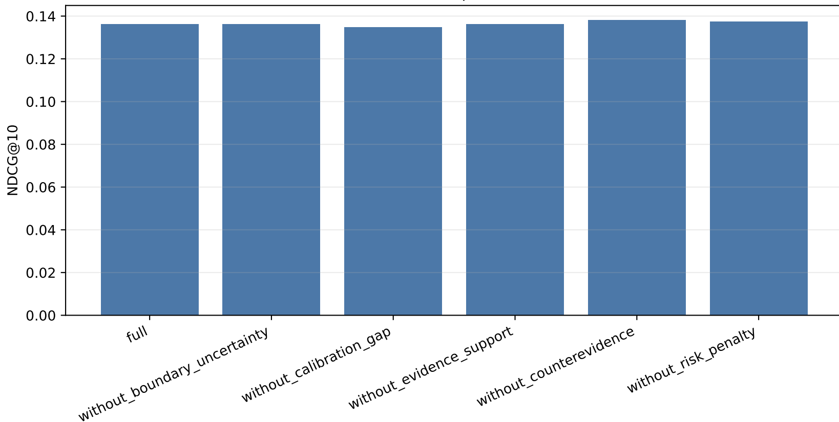
C-CRP leave-one-component-out ablation
