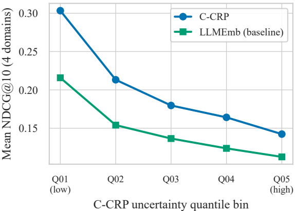
Ranking quality declines as uncertainty rises
