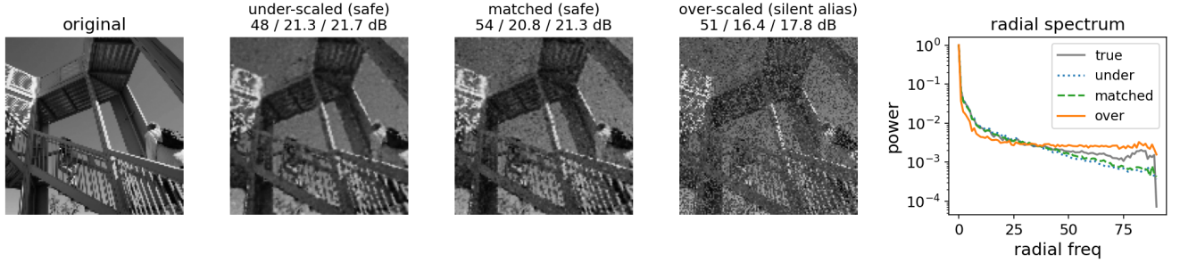
Fig. 4. The limit generalizes to a trained nonlinear 2-D INR fit to sparse image pixels (panel numbers: PSNR on the observed pixels / full field / upper radial-frequency band; figure: seed 0, metric ranges over three pixel-mask/noise draws). An over-scaled representable band silently aliases: it fits the observed pixels (49–64 dB) but the full field is moiré-corrupted (16.3–16.6 dB) and its radial spectrum carries spurious high-frequency energy; a band matched to (or below) the sampling is safe—under- and matched-band fits are comparable across draws (full-field 20.8–21.4 dB); the contrast that matters is with the over-scaled band.
