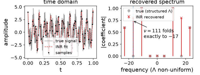
Fig. 1. Silent aliasing onto a structured \Lambda = \{0, \pm 5, \pm 11, \pm 17, \pm 23\} ( m=9 ): the exact-fold regime of Thm. 2(iii). N=96 nonuniform samples (a random subset of a rate- Q=128 grid, N \gg m ), noise \sigma=0.03 . The INR fits the samples at the noise floor (RMSE 0.026; 0.028 \pm 0.002 over 20 draws) yet its reconstruction error is 1.60 and its spectrum carries the full tone energy (bias 1.13): the tone \nu=111 folds exactly onto the non-classical atom -17 in every draw, while the true tones ( \pm 11, \pm 23 ) are kept. The fold appears on both \pm 17 (Hermitian pair of the real tone).
