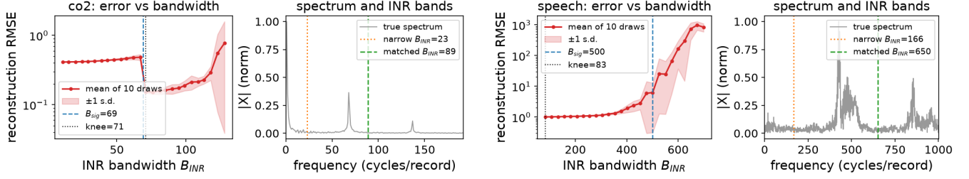
Fig. 3. Both sides of the limit on real data (curves: mean \pm 1 s.d. over 10 subsample/noise draws; dashed line B_{\text{sig}} = essential bandwidth, dotted line = error knee). Left ( \text{CO}_2 , recoverable): the knee sits at the annual-cycle frequency; a narrow INR aliases, a matched INR recovers (the mild rise past the knee is the onset of the noise gain). Right (speech, converse): the error never approaches the noise floor at any width—a truncation-plus-aliasing floor for narrow bands, and a noise-gain blow-up ( \kappa = 1/\sigma_{\min} \rightarrow \infty ) as the width approaches the sample budget.
