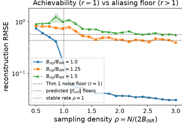
Fig. 2. Achievability vs. converse (Thms. 1–2), 40-trial Monte Carlo (bands: \pm 1 s.e.), r = B_{\text{sig}}/B_{\text{INR}} , sampling density \rho = N/(2B_{\text{INR}}) . In-band ( r=1 ) error is large in the rank-deficient regime \rho < 1 , drops sharply at the stable rate \rho=1 , and then tracks the exact Thm. 1 noise floor (dashed); out-of-band ( r>1 ) error plateaus at the predicted \|f_{\text{out}}\| levels (dotted) that no density removes.
