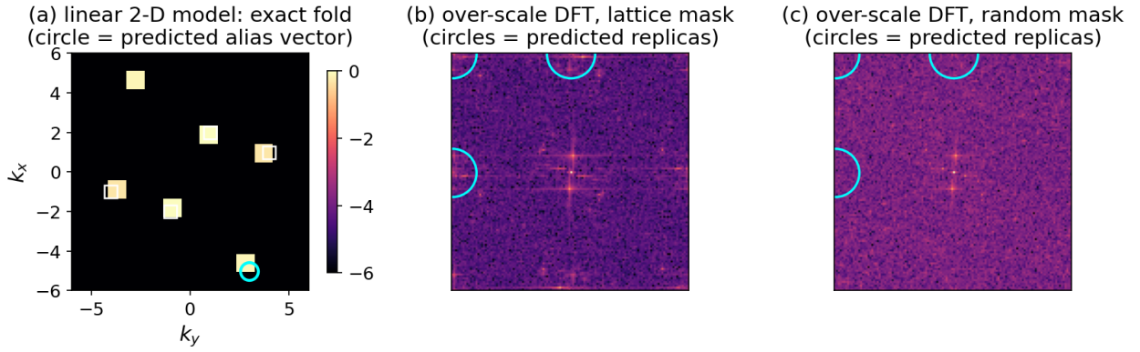
Figure 3: 2-D exact fold (linear) and lattice-vs-random replicas (trained).
