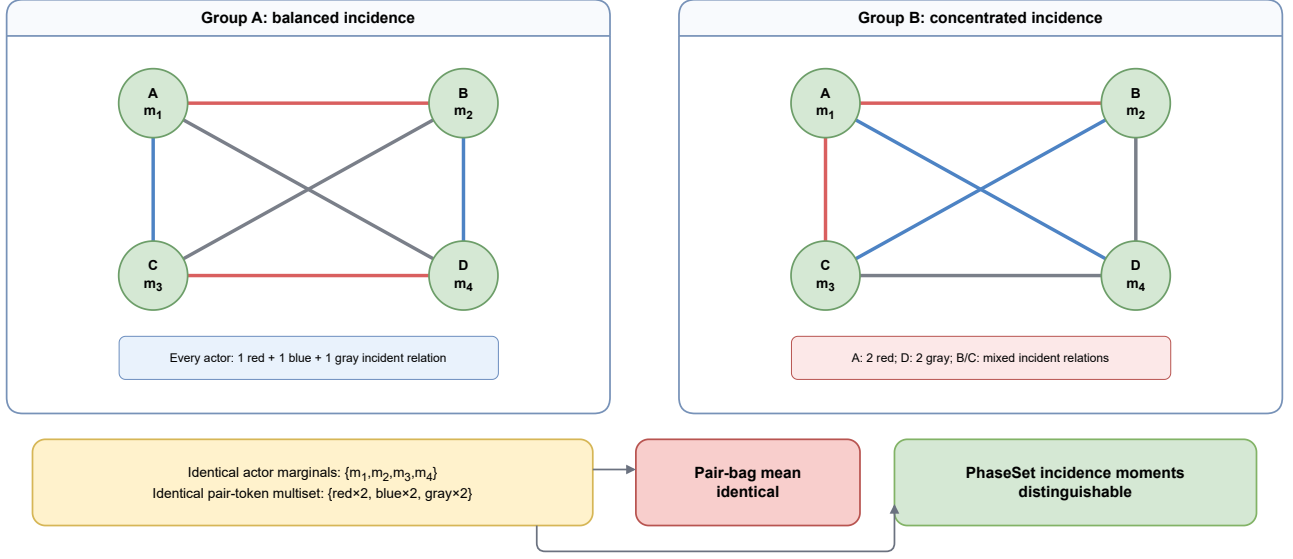
Fig. 1. Conceptual counterexample (not data or a result). Actor marginals and the pair-token multiset are identical, so pair-bag averaging cannot distinguish the groups; incident relation moments retain their different ownership.
