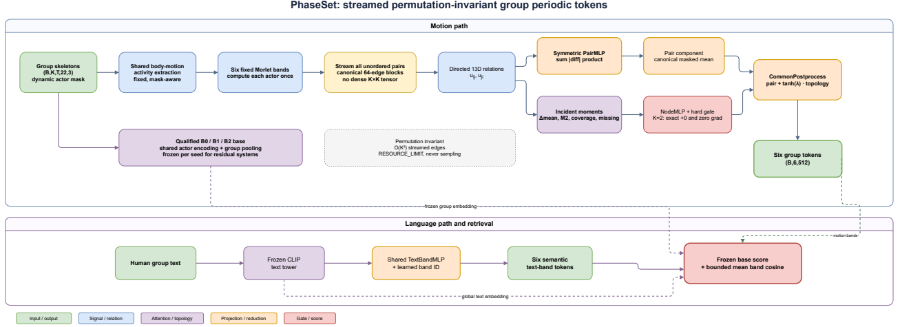
Fig. 2. Implementation architecture (no-result). Fixed motion activity and the qualified learned group base are parallel paths. Directed relations feed a symmetric pair mean and incident-moment topology path; a hard K=2 gate preserves dyadic equivalence. Six motion tokens align with six semantic text-band tokens on top of the frozen qualified base score.
