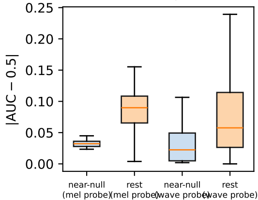
(b) near-null s_w stays at chance
