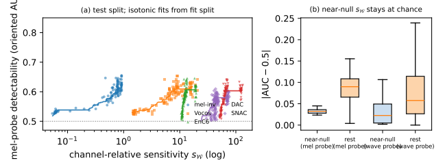
Fig. 1. E2, held-out test split. (a) Channel-relative sensitivity s_{\mathcal{W}} vs. mel-probe detectability, per attacker, with isotonic fits learned on the fit split. (b) Directions in the absolute near-null regime stay at chance in both probe domains.
