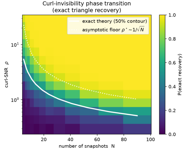
Fig. 1. Curl-invisibility phase transition for exact triangle recovery. Colour is empirical P(\text{exact recovery}) ; the solid line is the exact finite-sample law (Prop. 2), the dotted line the Bonferroni-corrected Chernoff floor of Thm. 1 ( \delta \rightarrow \delta/p ).
