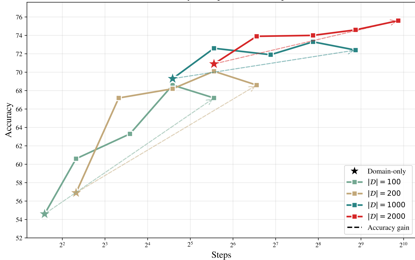
Accuracy vs. Optimization Steps
