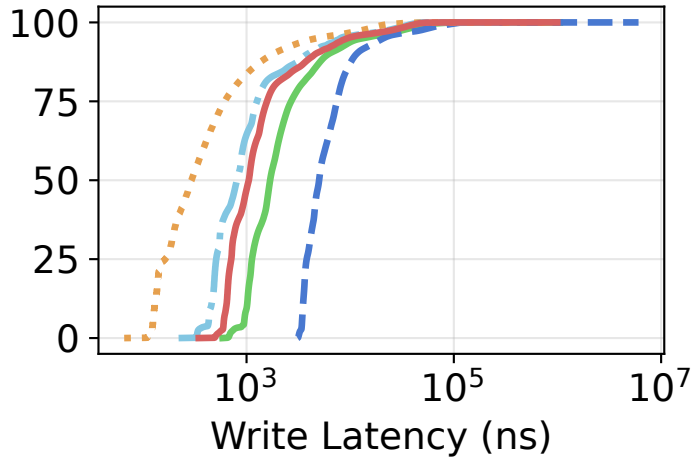
Hotel Reservation
