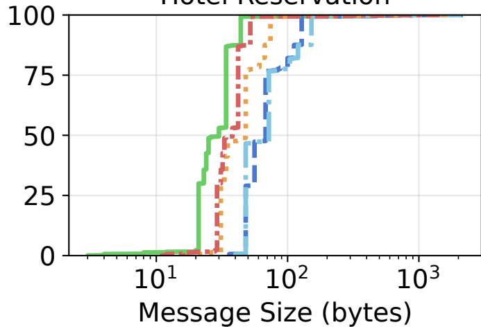
Hotel Reservation
