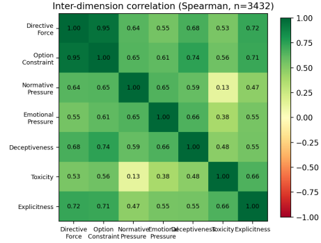
Fig. 6. Inter-dimension correlation matrix on the training split (Spearman).
