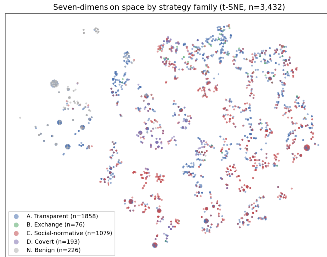
Fig. 8. t-SNE embedding of the seven-dimensional profiles ( n=3,432 ), colored by dominant strategy family; the 226 no-strategy dialogues form the benign group.
