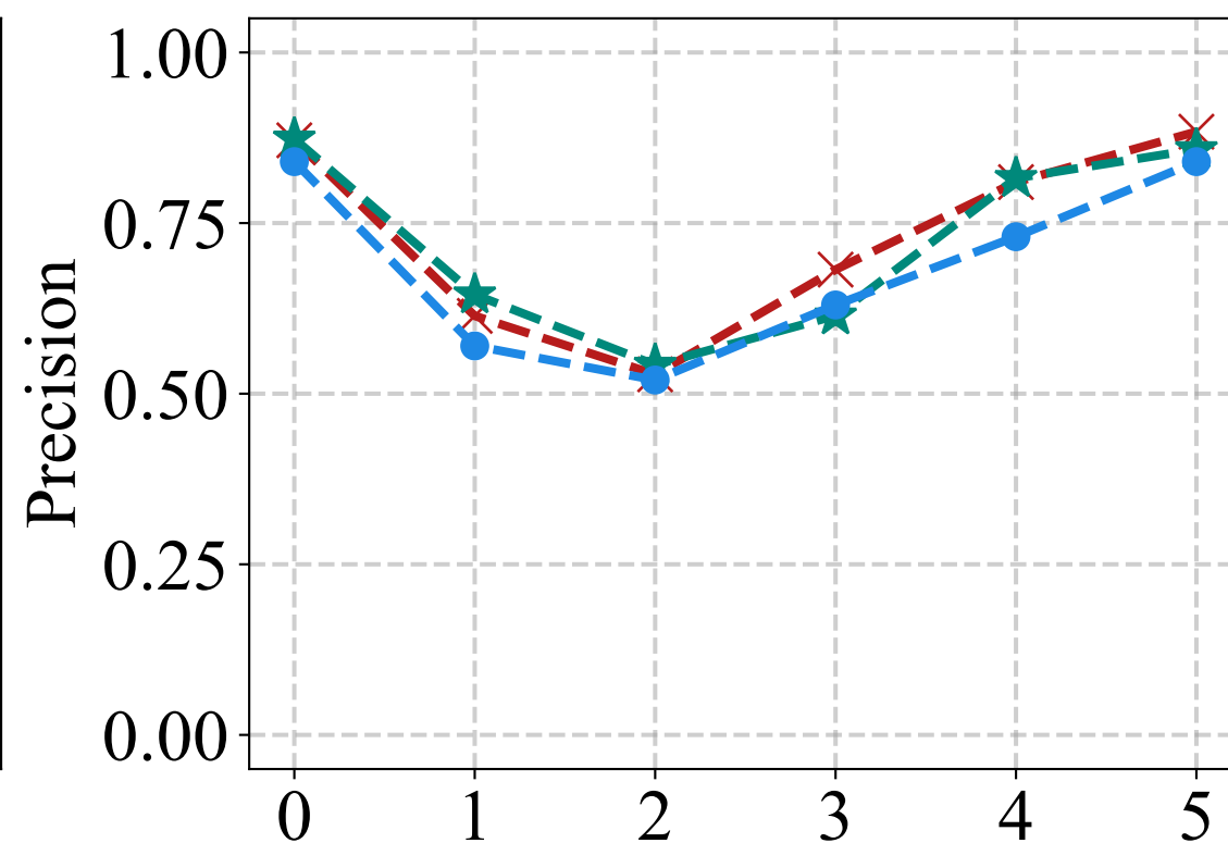
Fine-tuned: Precision
