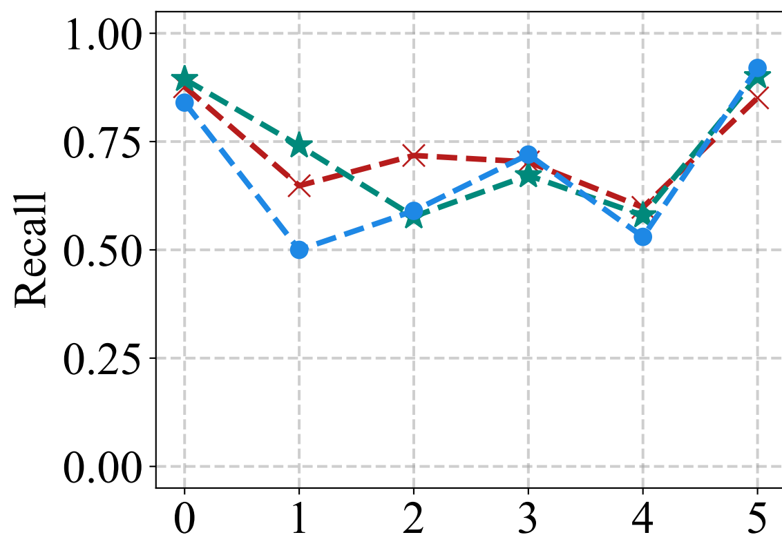
Fine-tuned: Recall
