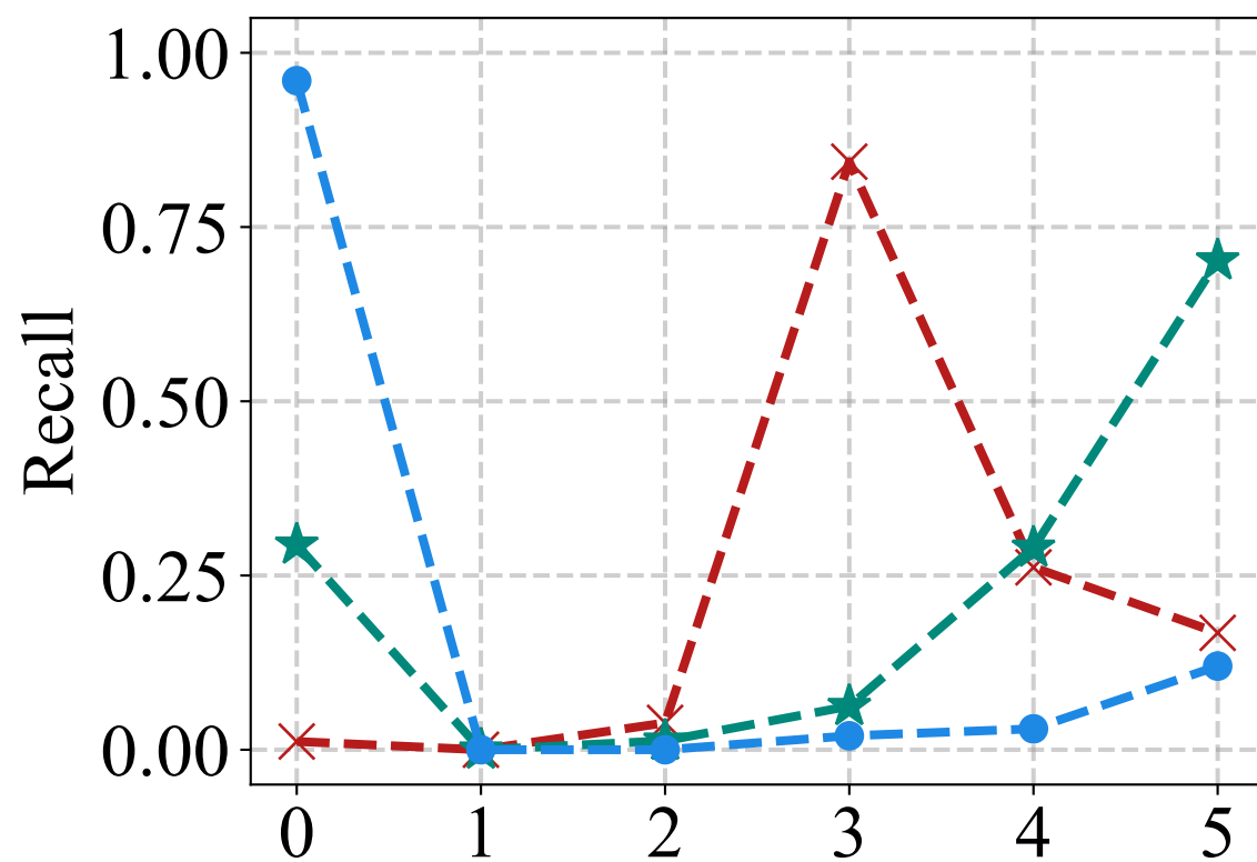
Zero-shot: Recall
