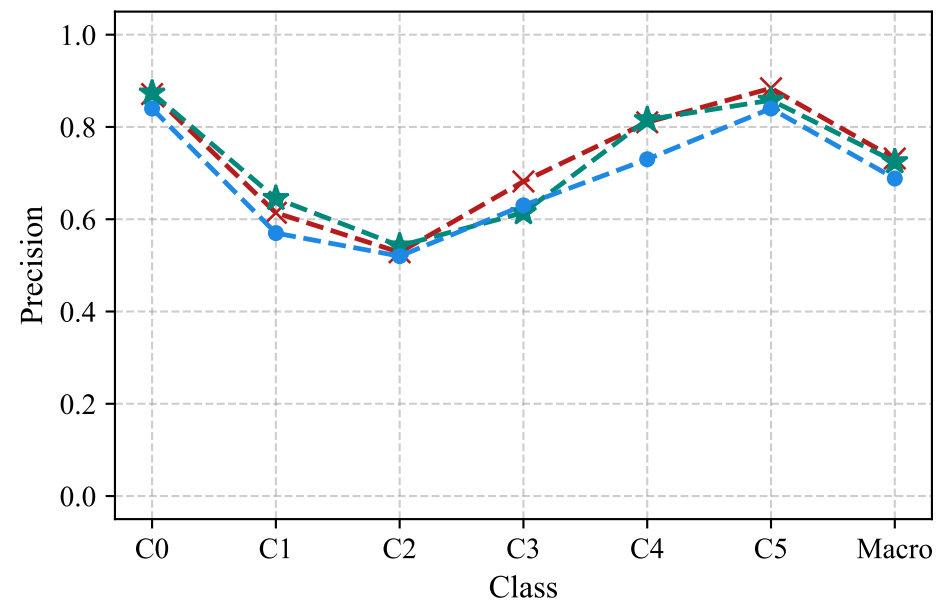
Fine-tuned: Precision
