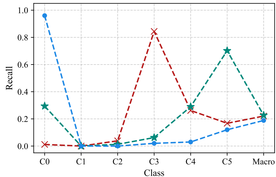
Zero-shot: Recall
