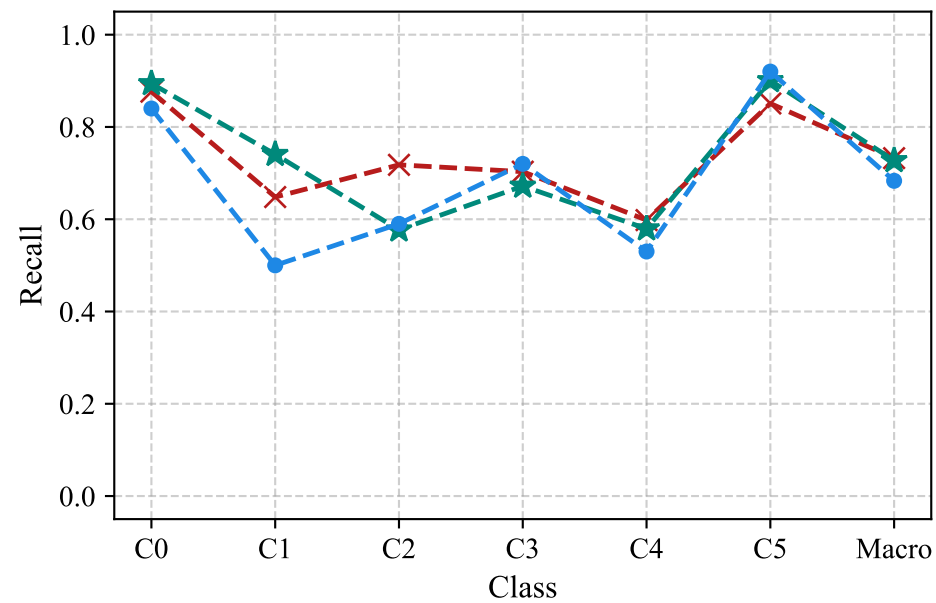
Fine-tuned: Recall
