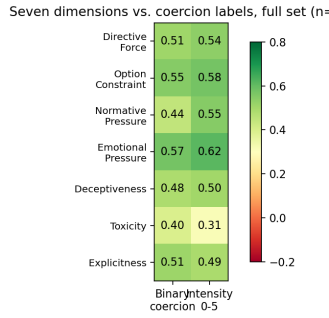
Fig. 3. Seven dimensions versus the binary and 0-5 intensity labels on the full release ( n=3,432 ; Spearman correlation).
