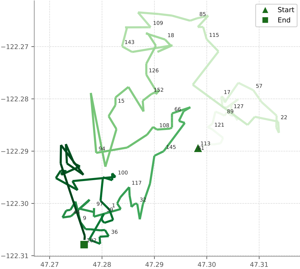
Hybrid Algo 2+5 (Delivery Stops Only) Cost: 13482.80
