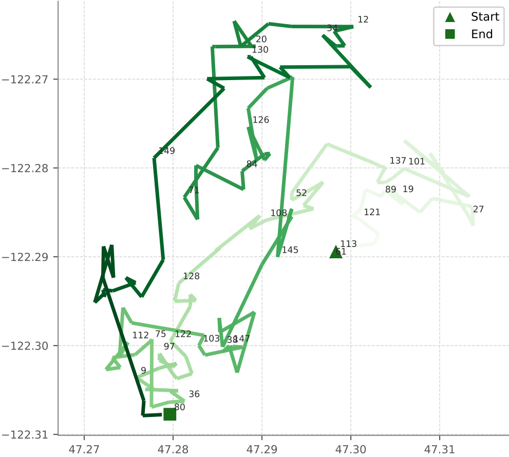
Hybrid Algo 2+5 (Delivery Stops Only) Cost: 15442.60
