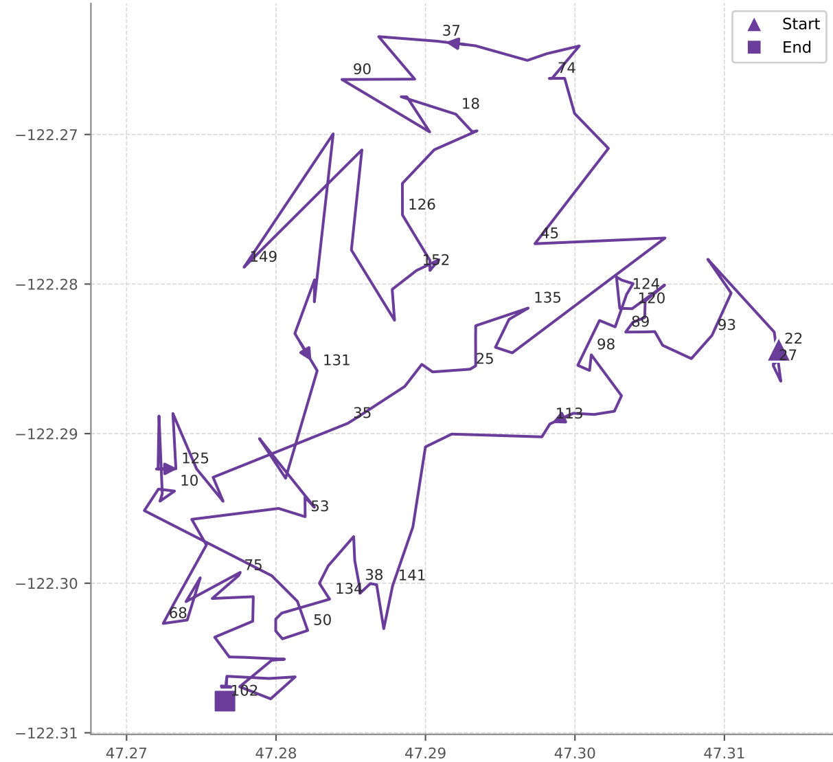
CG Hybrid (LRWSQAOA-Sub) (Delivery Stops Only) Cost: 13884.20
