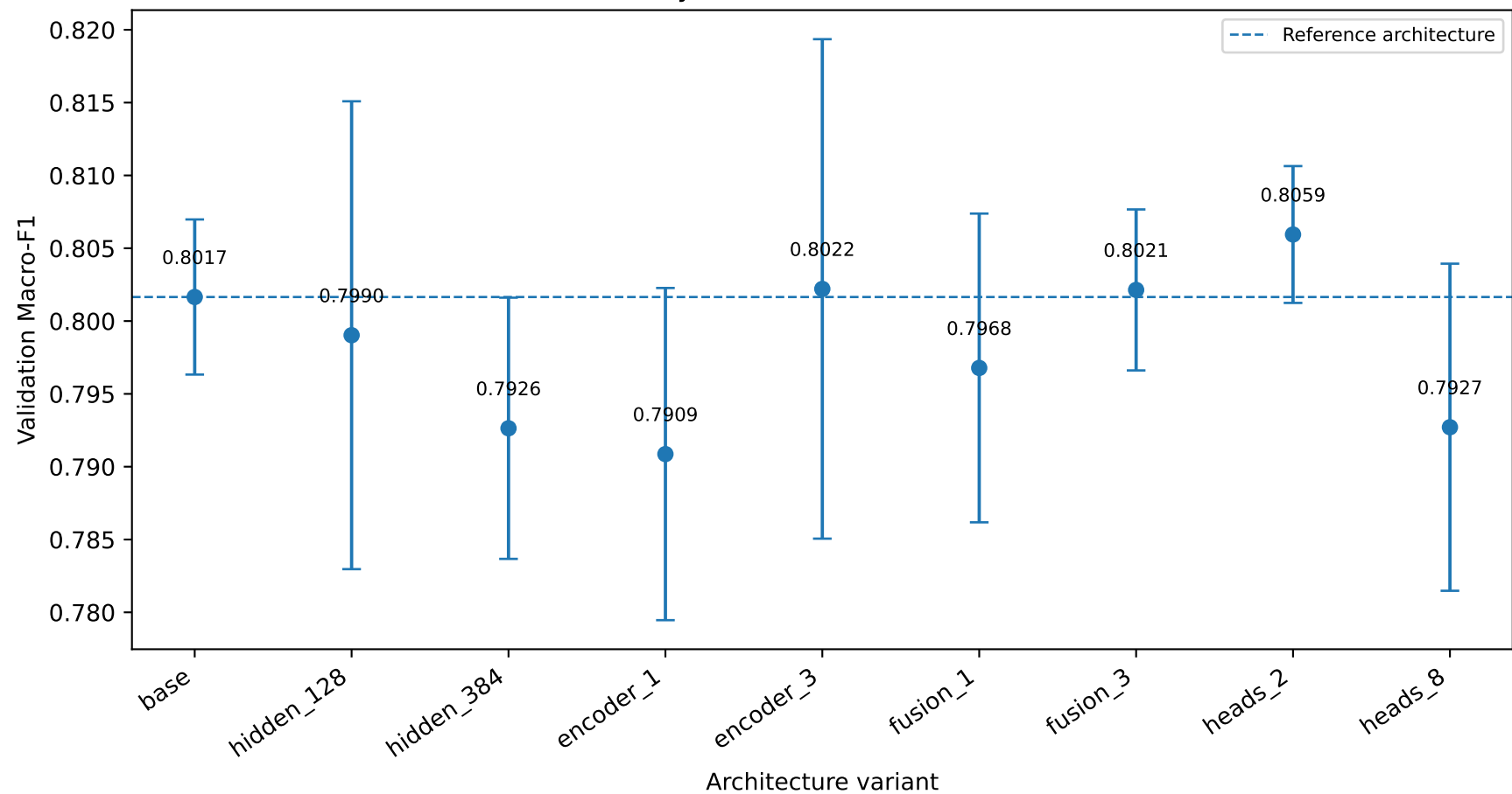
Architecture sensitivity on validation data (3 seeds; mean \pm SD)
