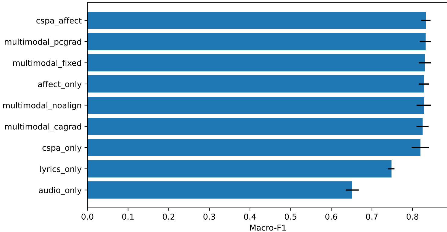
Emotion prediction performance
