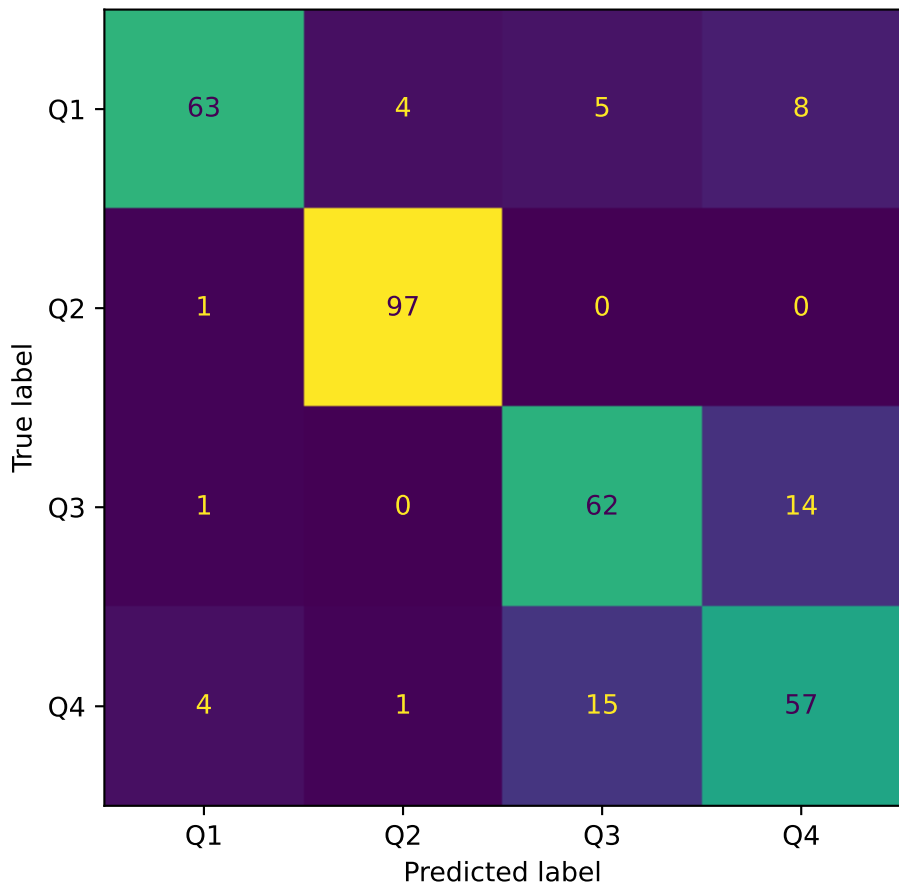
Final held-out test confusion matrix
