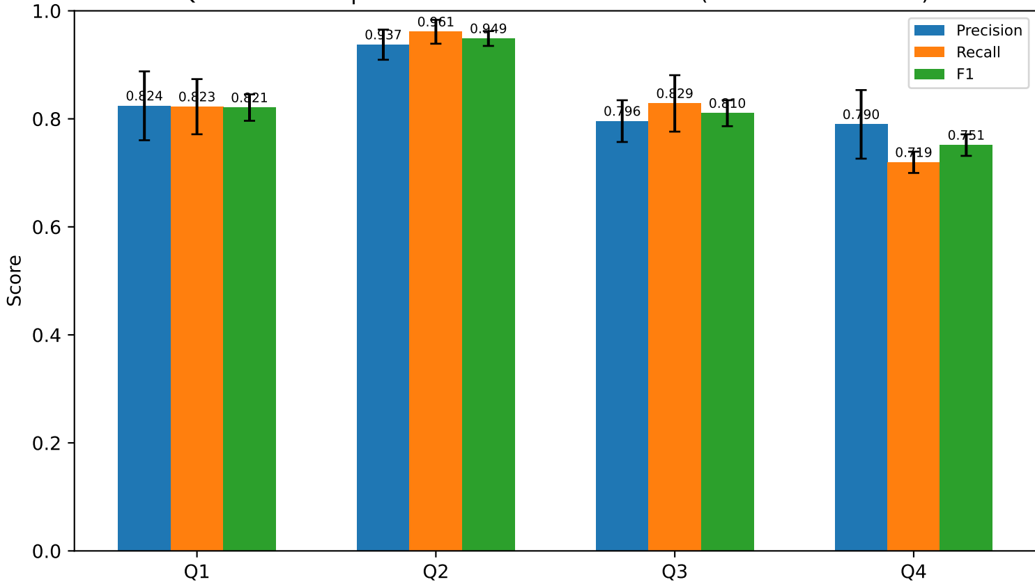
Quadrant-wise performance for CSPA + affect (five held-out seeds)
