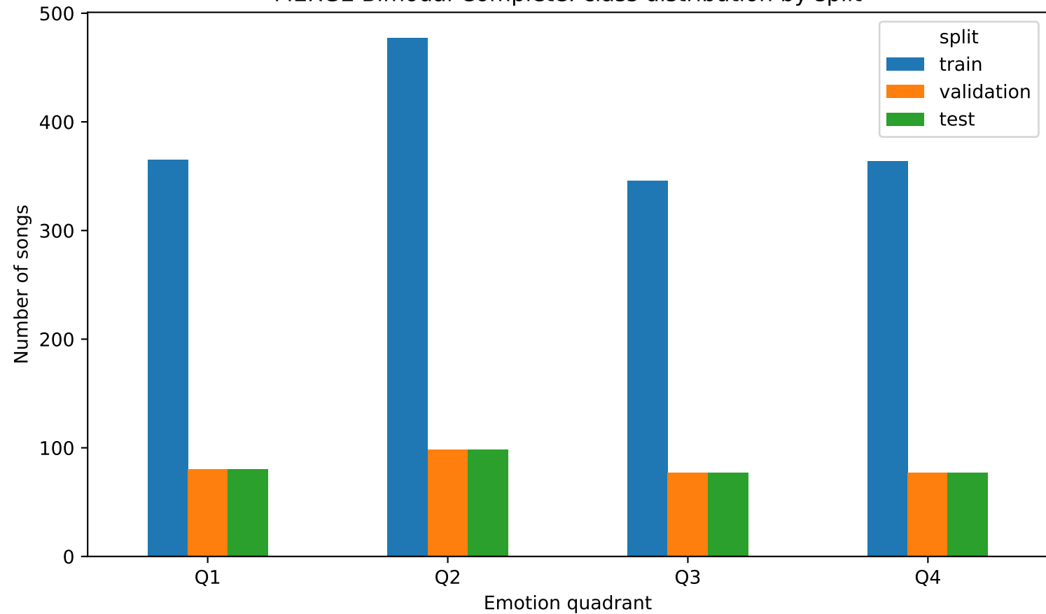
MERGE Bimodal Complete: class distribution by split
